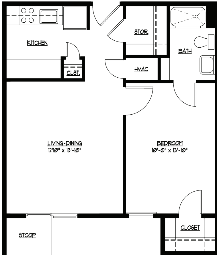
One Bedroom Floor Plan 522 Total Square Feet
